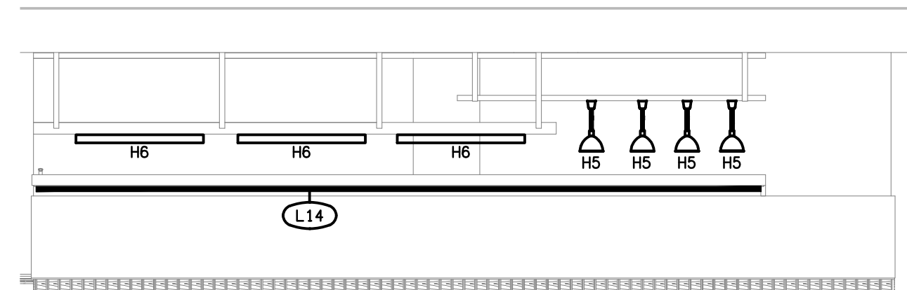
DETAIL D SERVERY COUNTER ELEVATION SCALE 1:50
